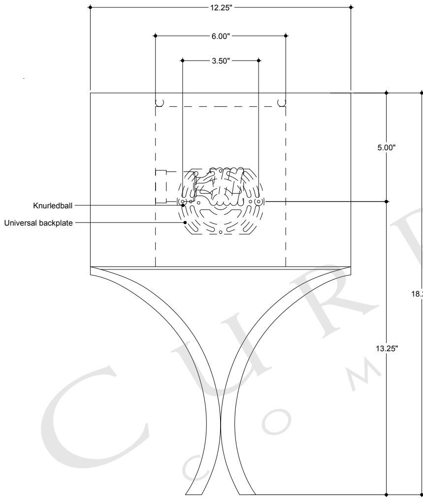
FRONT VIEW
