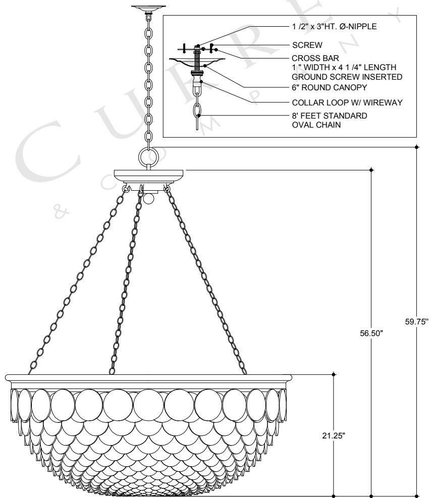
FRONT VIEW
