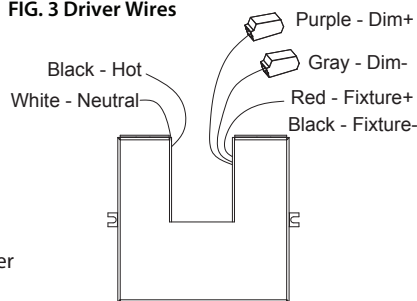
FIG. 3 Driver Wires
