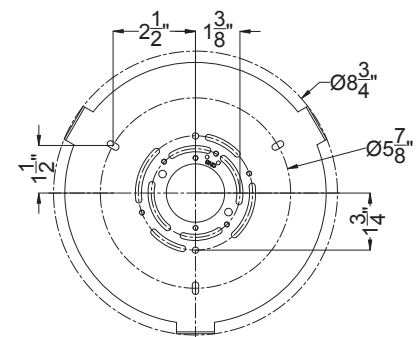
PD-59922/PD-59933 Back Plate
