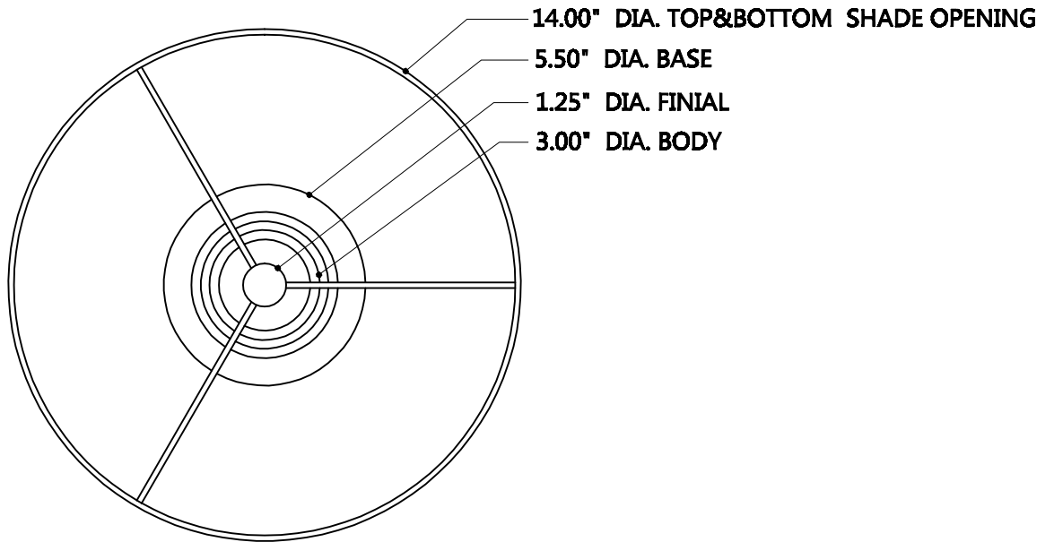
TOP VIEW
