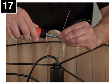
17 Tighten both screw of strain relief and adjust aircraft cable length as needed. Cut loose aircraft cable if necessary.
