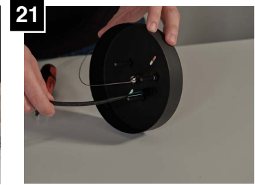
21 Pass power cord through strain relief (black) and twist to tighten power cord. Adjust length of power cord prior to tightening.
