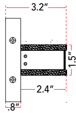
Side Elevation
