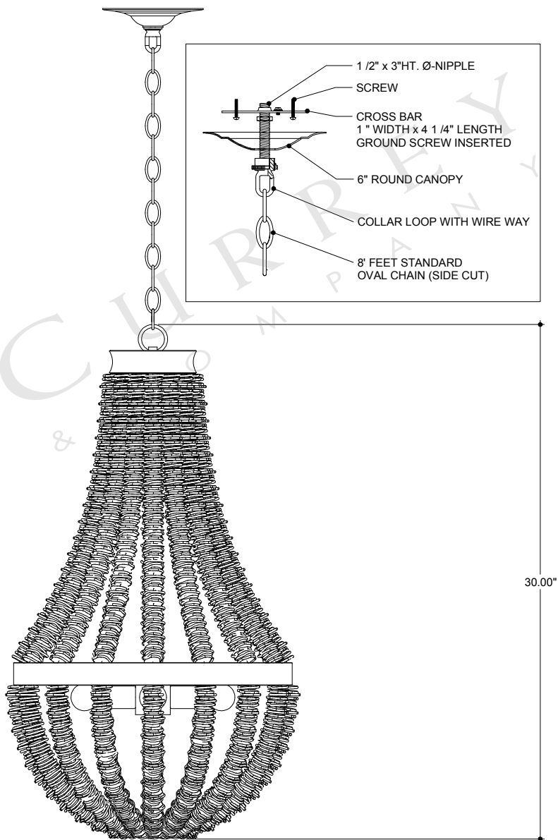
FRONT VIEW
