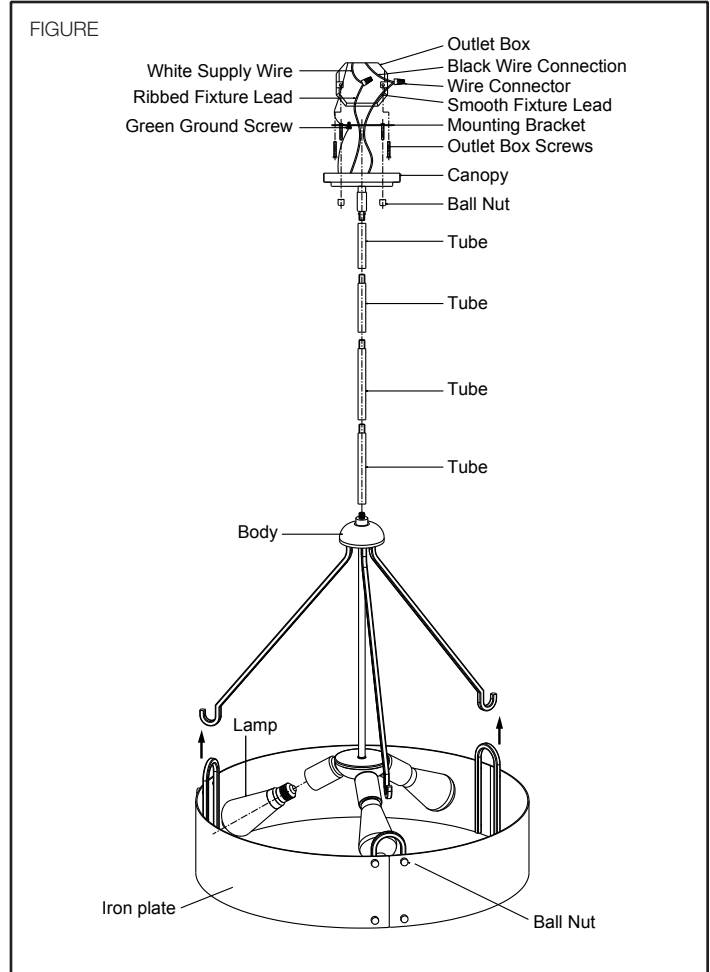
FIGURE Line art shown may not exactly match the fixture enclosed. However, the installations do apply to this fixture.
