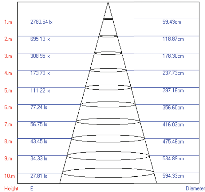
Lux-Distance Curve
