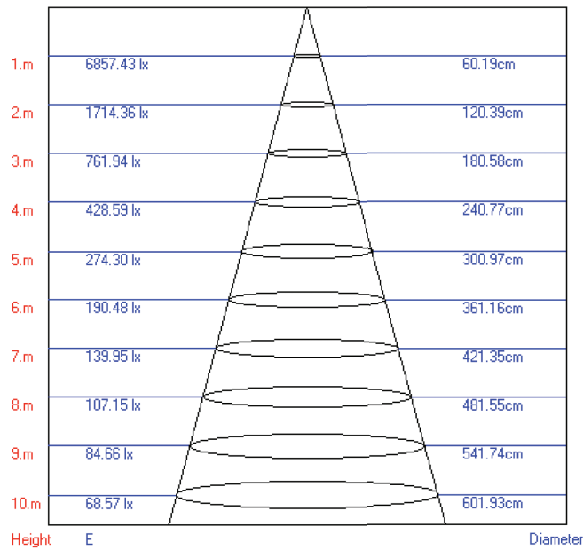
Lux-Distance Curve
