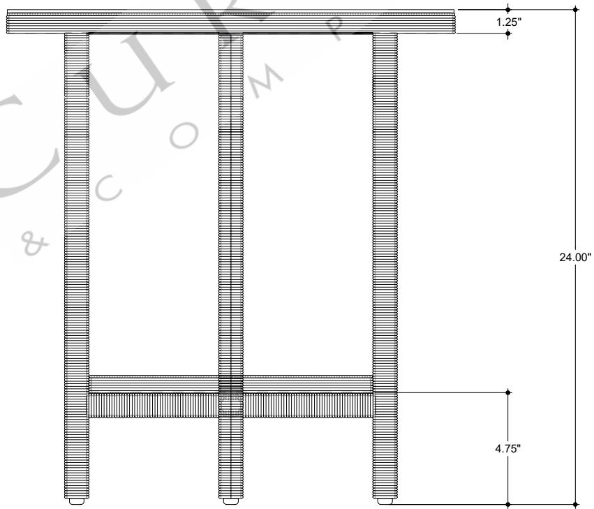
FRONT VIEW
