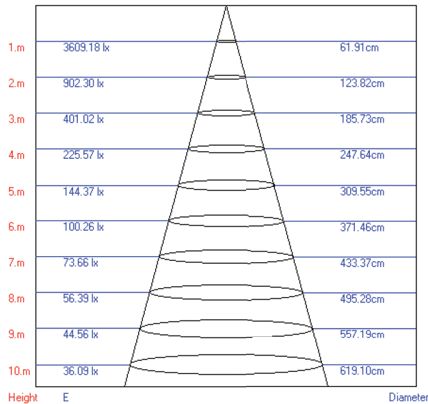
Lux-Distance Curve
