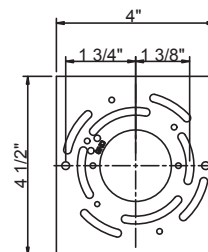
Back plate Dimensions
