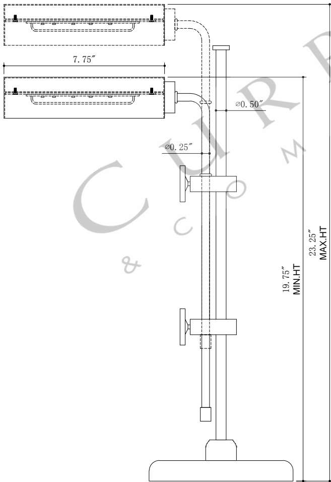
SIDE VIEW
