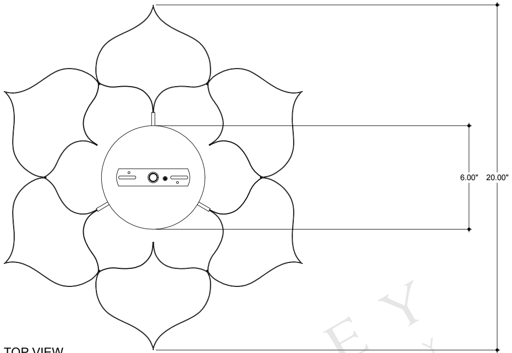
TOP VIEW
