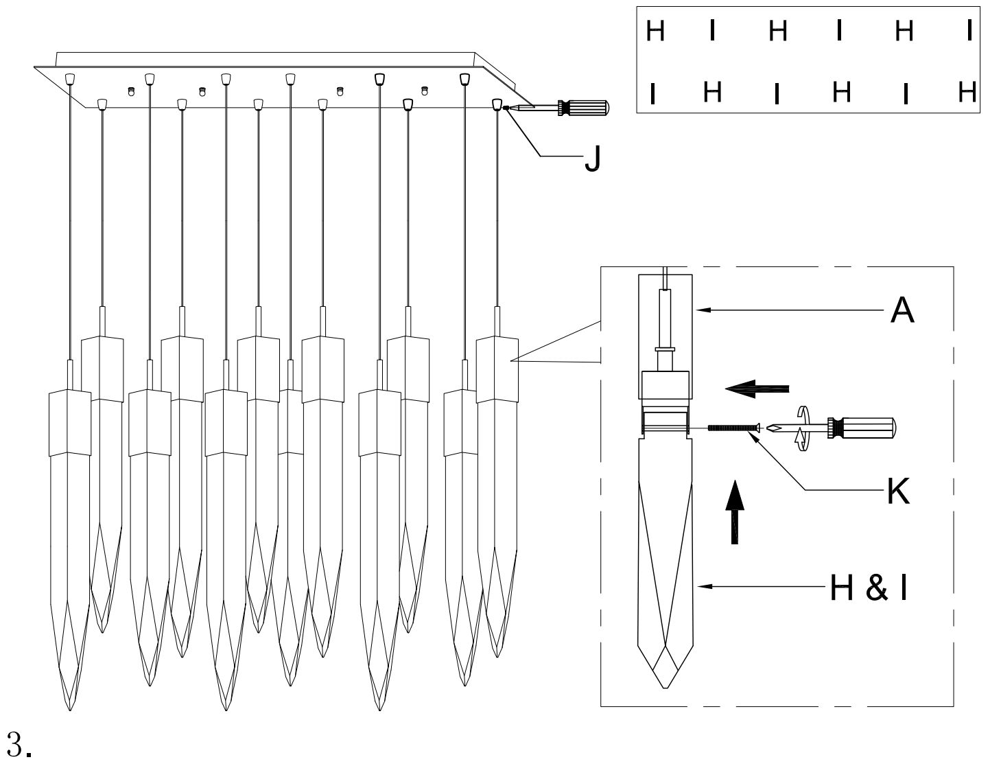
Schematic diagram of glass installation position
