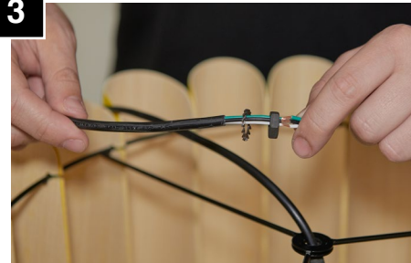
Pass lock washer and nut through cable.
