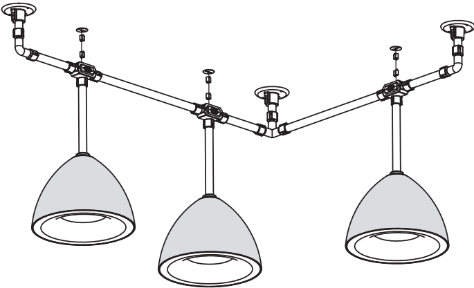
90° Corner Layout Example
