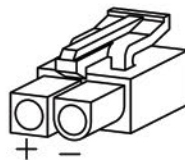
DLST42-5 - 18 AWG wire extension 152cm (5') complete with one male and one female connector - Please note polarity on each connector - Designed for use in Class II installation only
