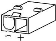
DLST42 - 18 AWG wire harness allowing 4 light connections - Maximum length 137cm (54"), distance between connectors 40cm (16") - Please note polarity on each connector - Designed for use in Class II installation only
