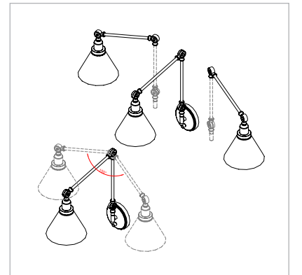
I. 9-9131CP-1-109 1-Light Adjustable Sconce Polished Nickel Finish 7-1/2"W x 17-1/2"H x 14"E Adj E 14" - 34-1/2" 1E 60W Clear Glass
