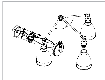
A. 9-960-1-89 1-Light Adjustable Sconce Matte Black Finish 5-1/2"W x 17"H x 13"E Adj E 13" - 33-3/4" 1E 60W
