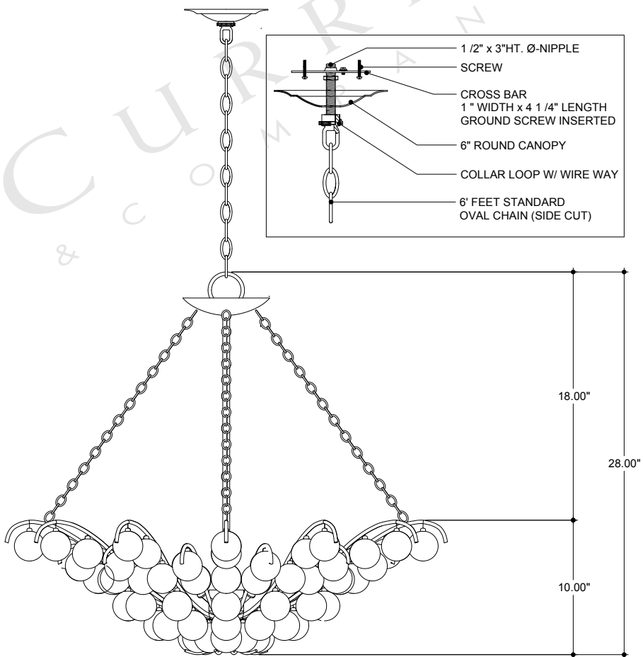
FRONT VIEW
