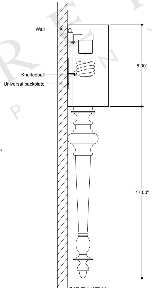
SIDE VIEW
