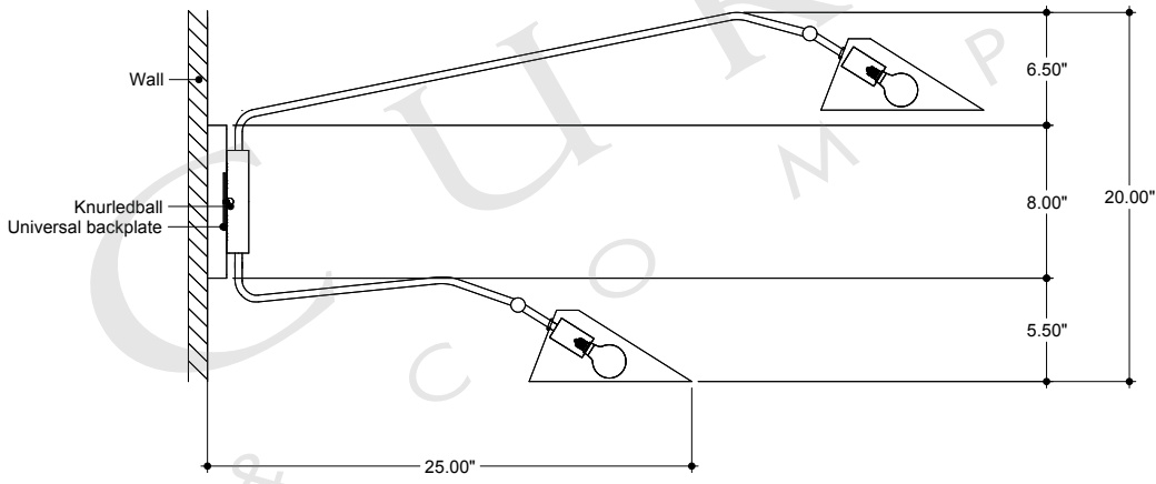
FRONT VIEW
