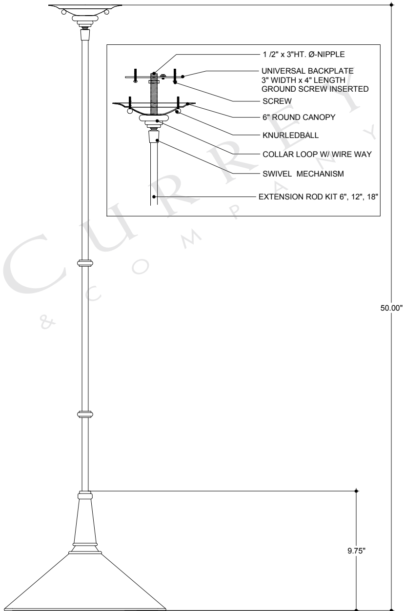
FRONT VIEW
