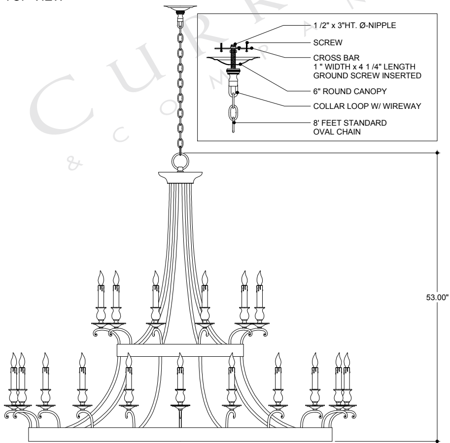
FRONT VIEW
