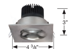
3 1/2" SQUARE - DOWNLIGHT
