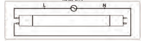
Single Ended Wiring Diagram AC120-277V
