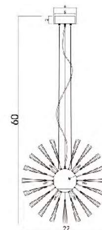
GA74S G4x12 (1.5W) LED
