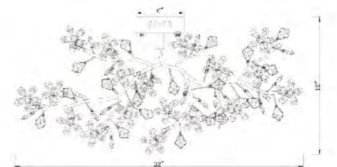
LX9907 (CLEAR+SMOKY CRYSTAL) G4×20 LED 3W DIMMABLE
