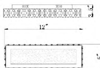
FT32W12CH LED 17W 4000K (Include)
