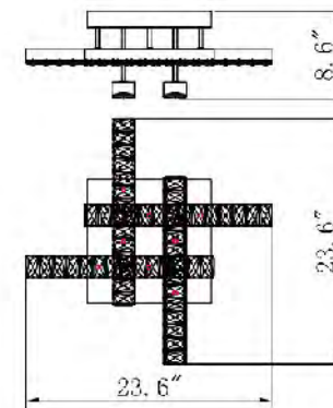
DIN07C23CH LED 32W (Include)
