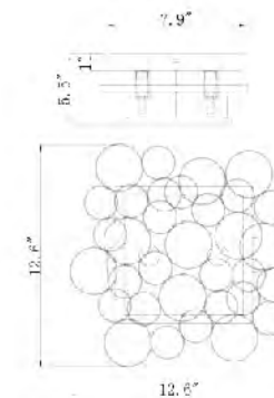
ZL22W12MN G9×4 Max40W
